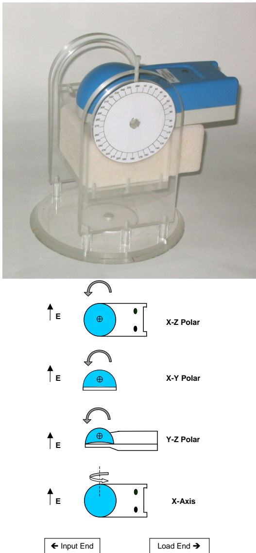
Figure 2 Jig and rotations used to examine isotropy of the PEM response
