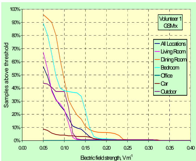
Figure 4 Example of processed personal exposure record results for the exposure of one volunteer in the GSMrx band
