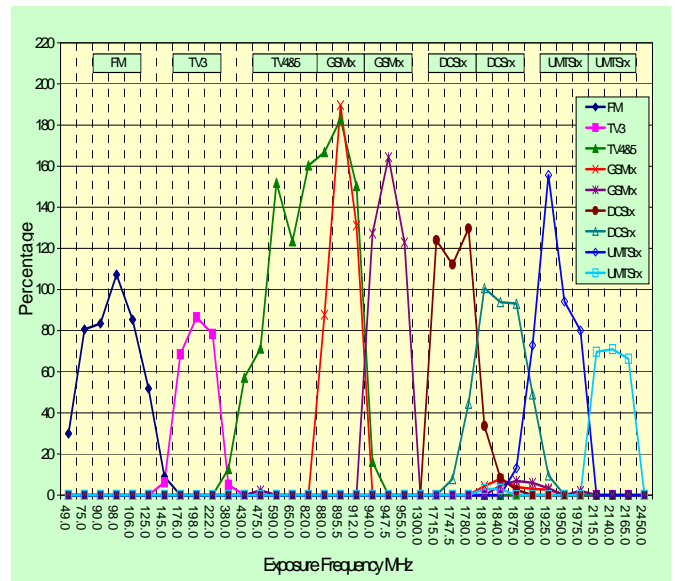
Figure 3 Relative response of a single axis of one PEM to an unmodulated field of 2.5 \text{ V m}^{-1}
